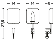
APEX CLIP LAMP WIDTH 14 CM DEPTH 8 CM HEIGHT 27,5 CM
